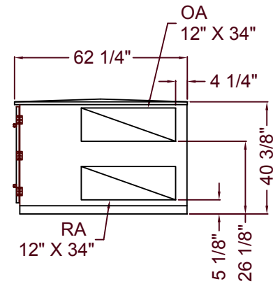
Right View
