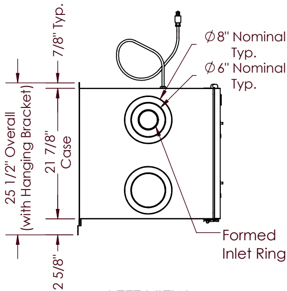
LEFT VIEW
