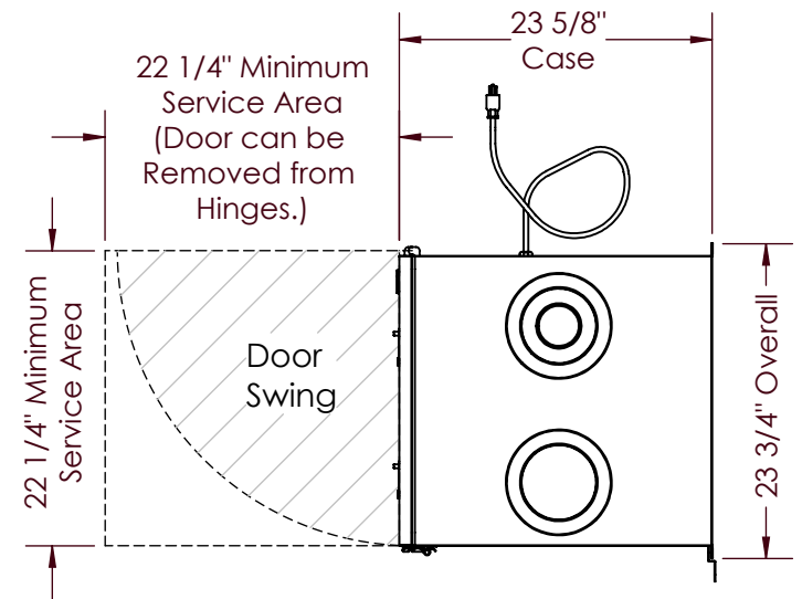
RIGHT VIEW
