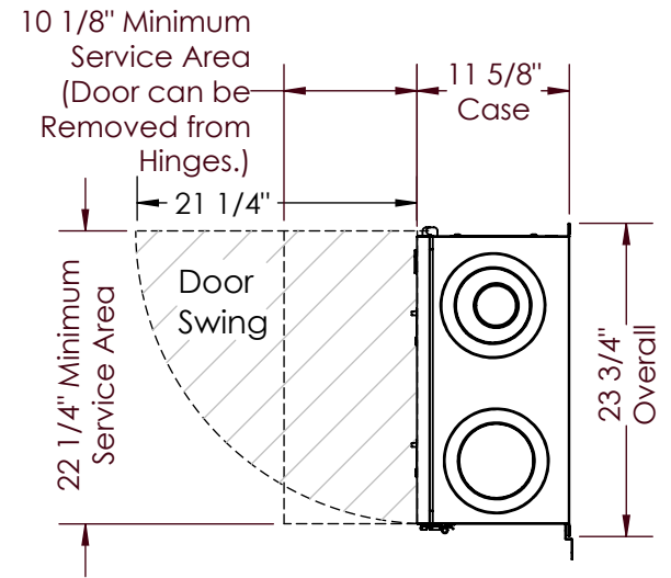
RIGHT VIEW
