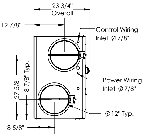
LEFT VIEW
