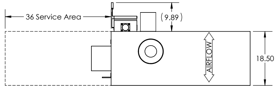
TOP VIEW
