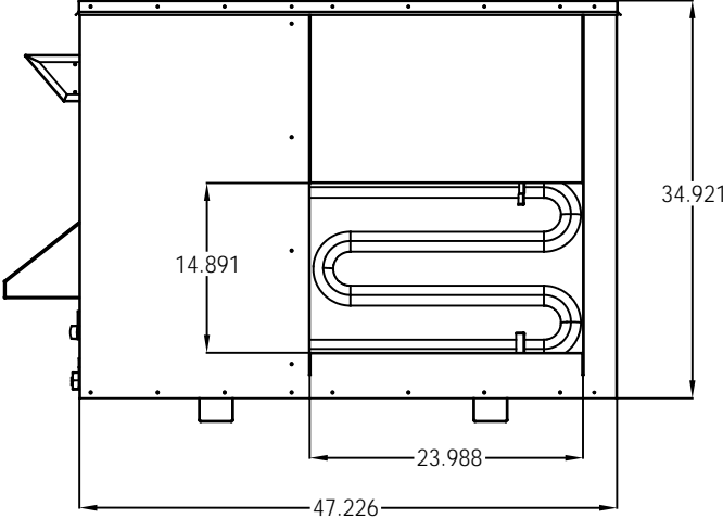
RIGHT VIEW
