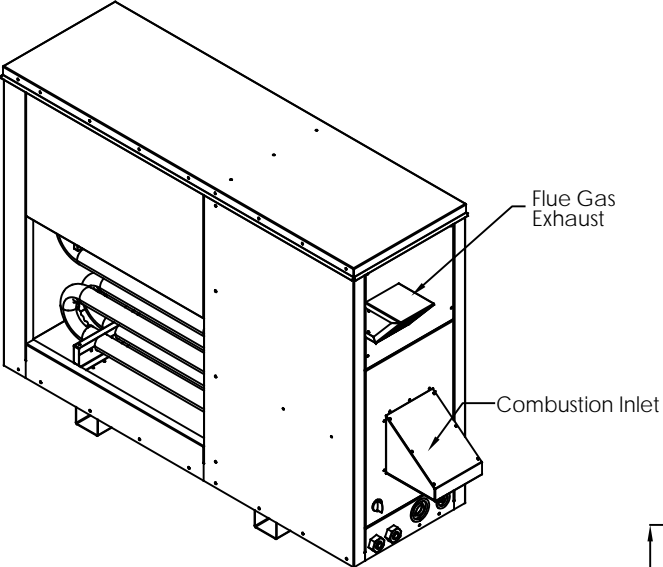
ISOMETRIC VIEW
