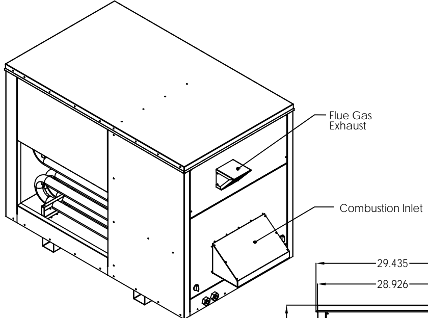
ISOMETRIC VIEW
