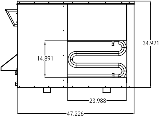
RIGHT VIEW
