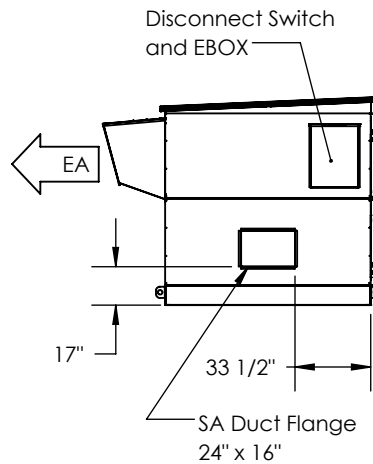
LEFT VIEW
