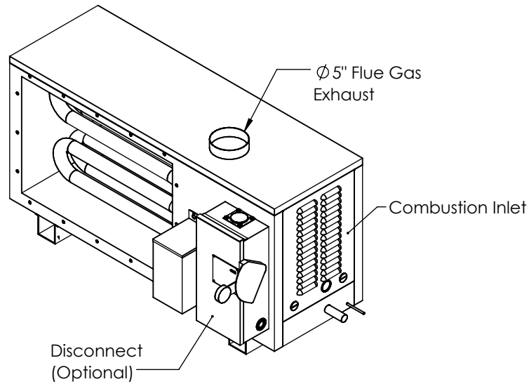
ISOMETRIC VIEW
