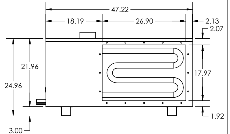
RIGHT VIEW
