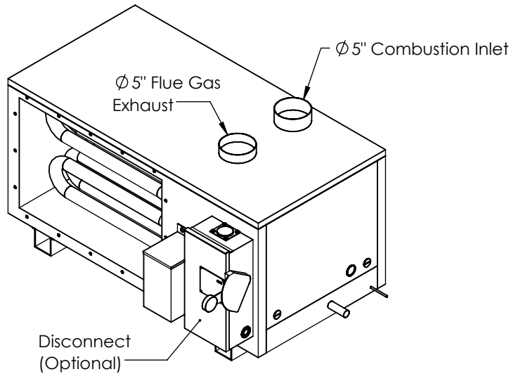
ISOMETRIC VIEW
