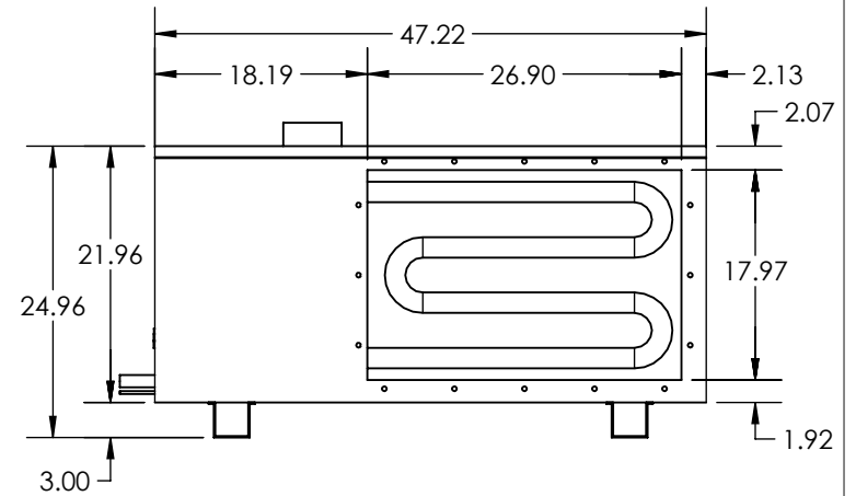
RIGHT VIEW
