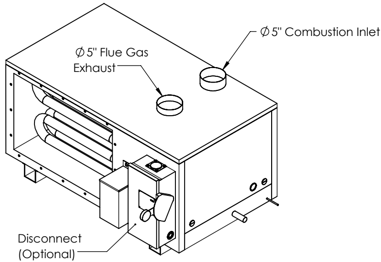
ISOMETRIC VIEW
