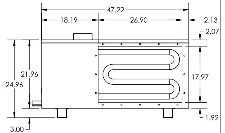
RIGHT VIEW
