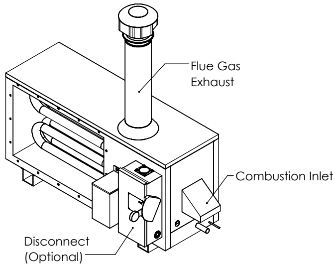
ISOMETRIC VIEW
