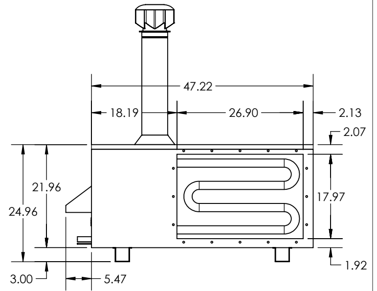
RIGHT VIEW
