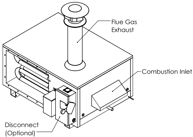
ISOMETRIC VIEW
