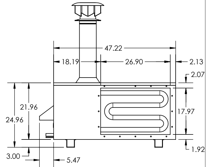
RIGHT VIEW
