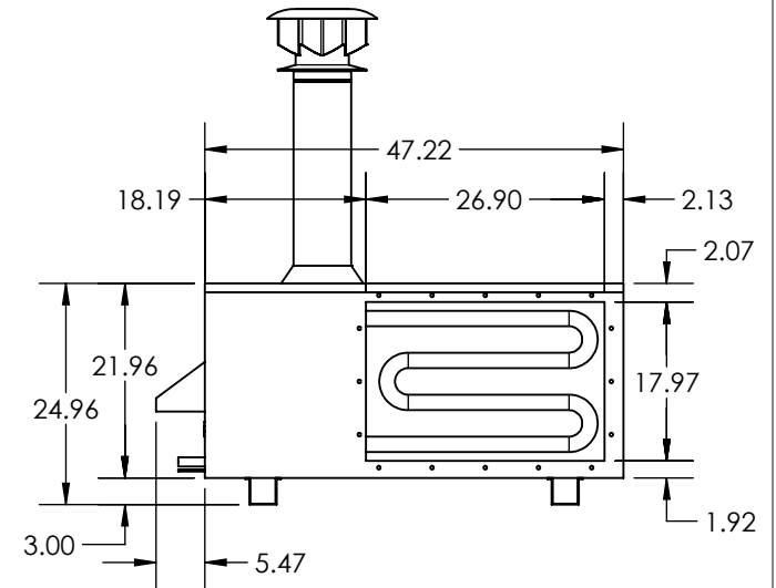
RIGHT VIEW
