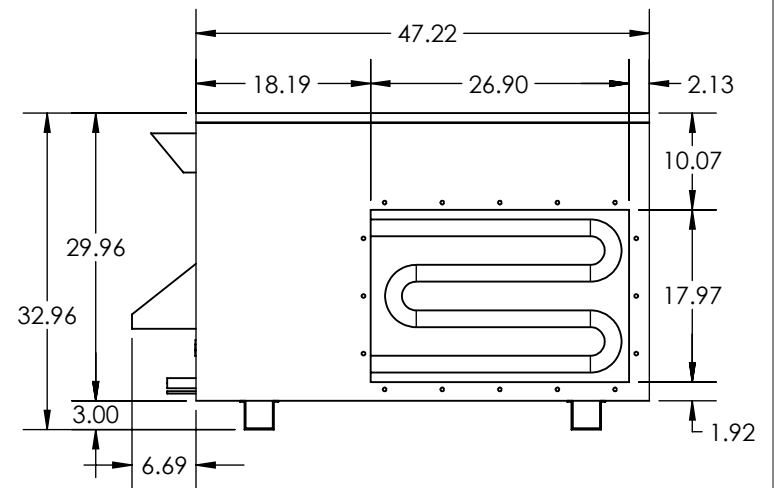
RIGHT VIEW
