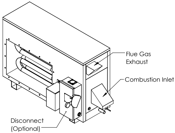
ISOMETRIC VIEW
