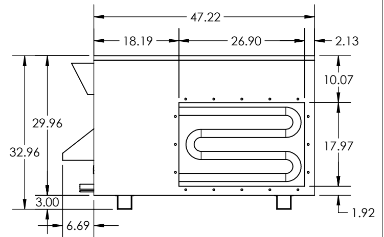
RIGHT VIEW
