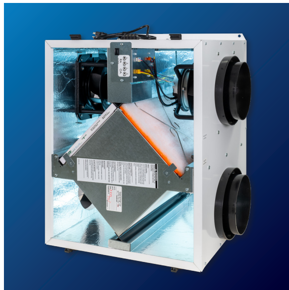
RenewAire introduces the EV Premium X ERV to its award-winning EV Premium Series product line. The X provides energy recovery ventilation to small/medium commercial spaces under 3,500 sq. ft. and large residences surpassing 5 bedrooms and 4,000 sq. ft.
